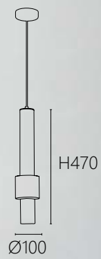
OK 21481 36000 Ø100 H470mm 線長1500mm LED 5W x 1 / MR16 x 1 3000K 鋁材
