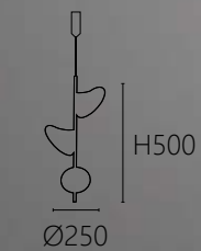
OK 21421 48000 Ø250 H500mm 線長1000mm LED 10W x 3 3000K 鋁材烤漆 壓克力
