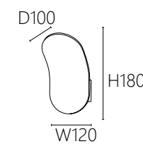
OK 20092B/W 12500 W120 H180 D100mm 內附LED 6W 3000K 鋁材烤漆
