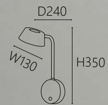
OK 20521 32000 W130 H350 D240mm 附LED 8W x 1 3000K 鋼材 附開關
